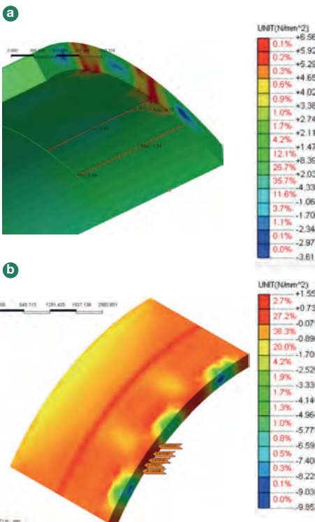
Figure 13 : Bursting and spalling tensile stresses developed in segments due to TBM thrust jack forces and gasket pressure: (a) transverse stresses; and (b) radial stresses (Bakhshi and Nasri 2013b; 2014d).
