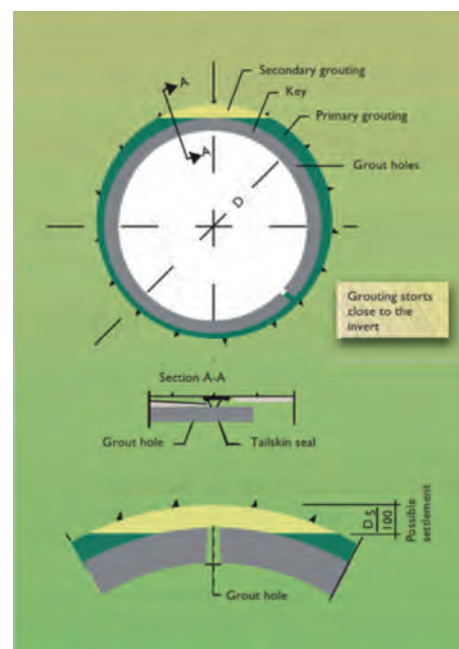
Figure 17 : Secondary grouting through segment grout hole (Guglielmetti et al. 2007).
